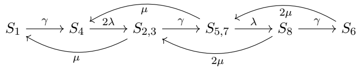
Fig. 15: Aggregated process for S .
